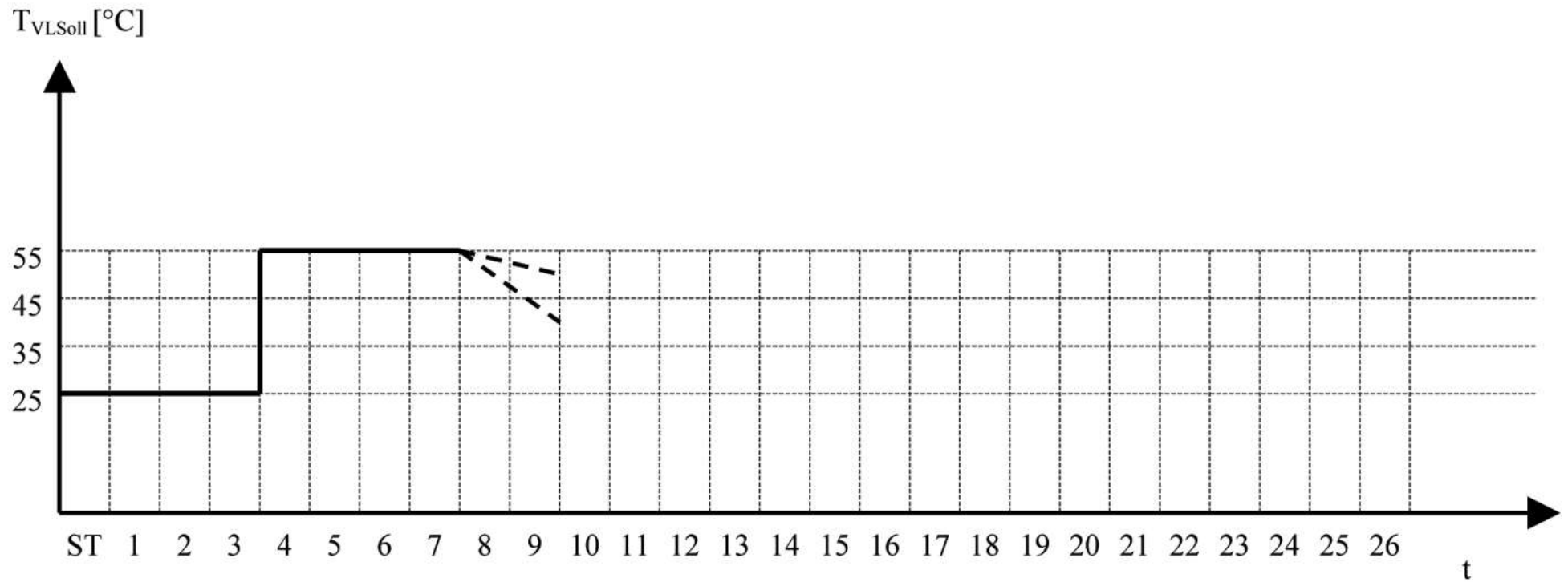
Fig. 50: Time sequence - functional heating
