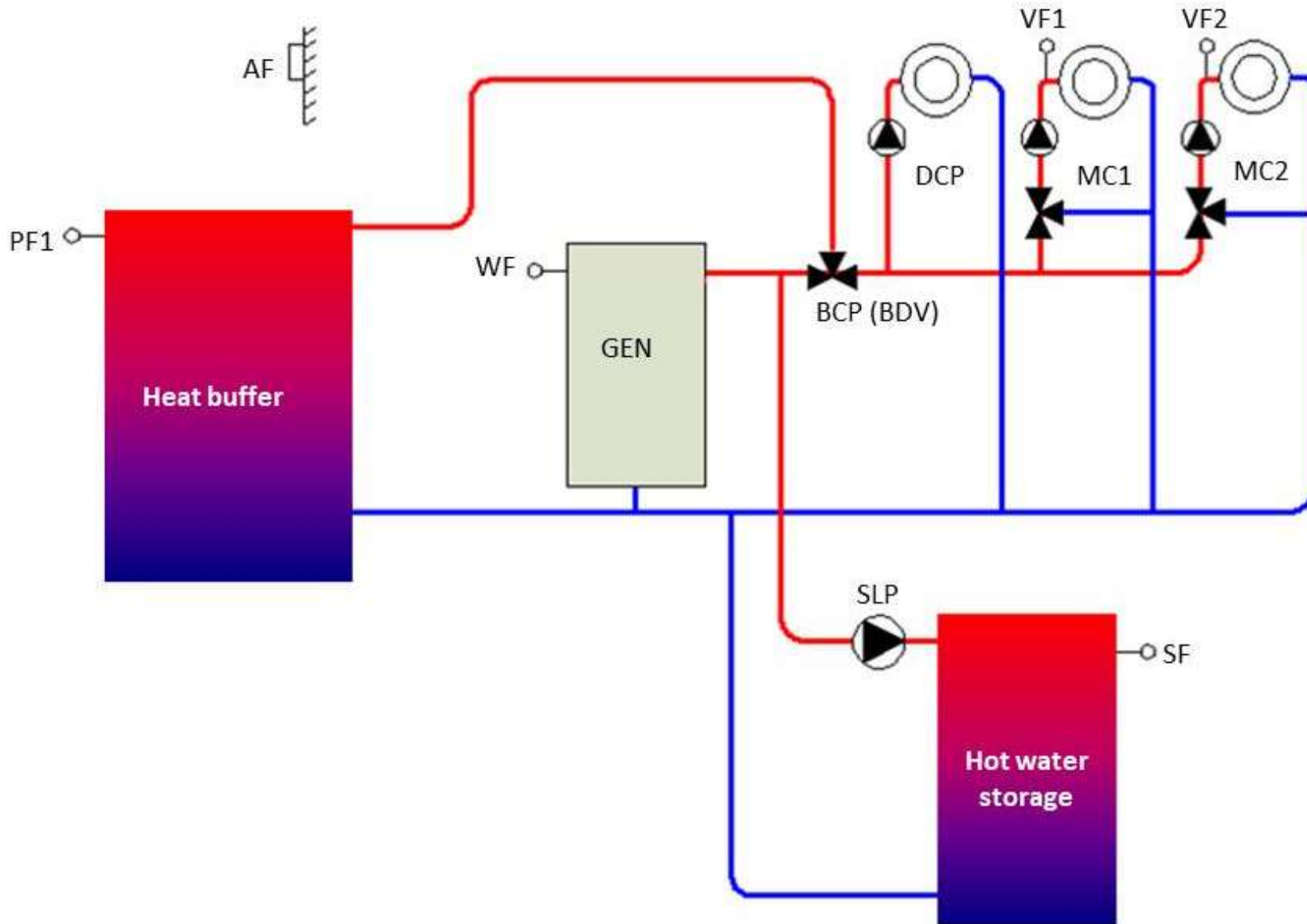
Fig. 61: Buffer discharge control on HC
