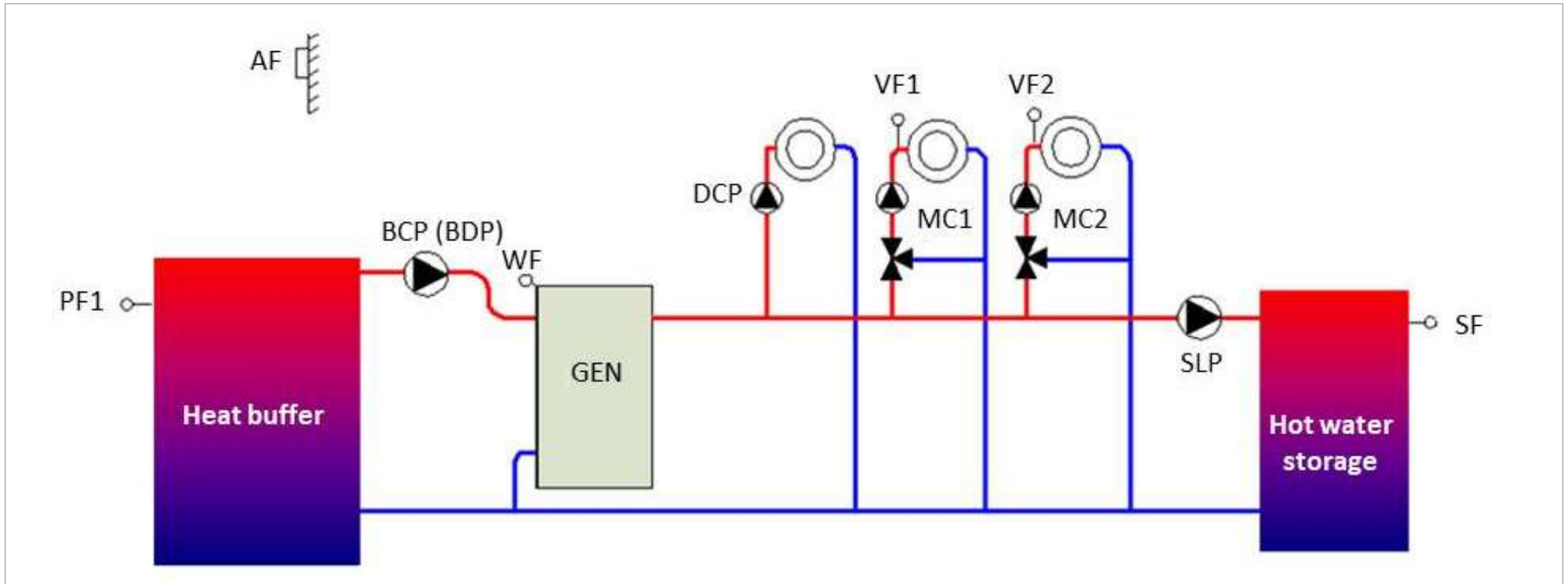
Fig. 62: Buffer discharge control type 2 on heat generator
