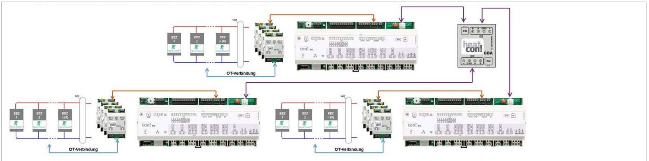
Fig. 38: OpenTherm Cascade fully equipped
