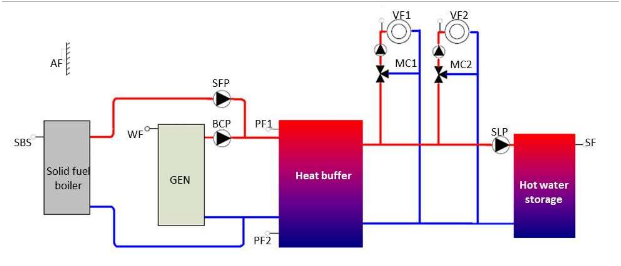
Fig. 57: Buffer charge control with solid fuel boiler for heating circuit and hot water
