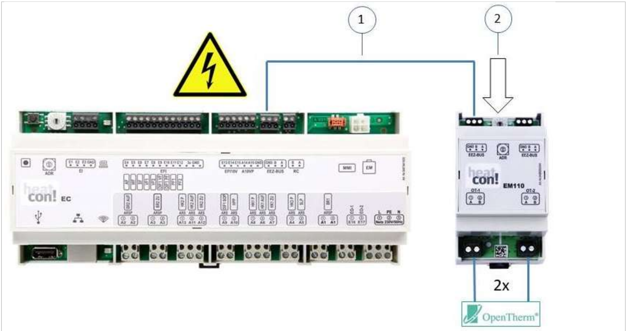
Fig. 8: Connection heatcon! EM 110 - OT to the heatcon! EC 1 GEN-Bus 2 Adress-switch
