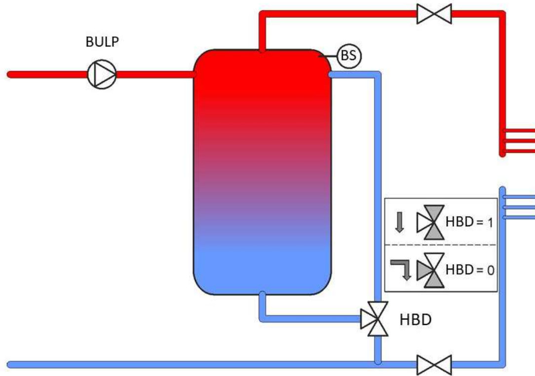
Fig. 54: Example hydraulic scheme, Hydraulic buffer discharge HBD
