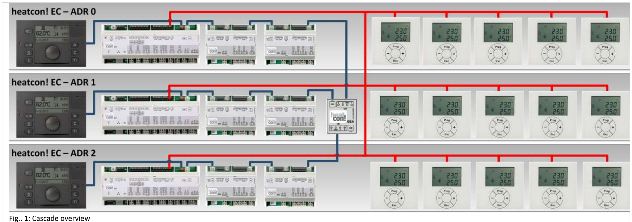
Fig.. 1: Cascade overview
