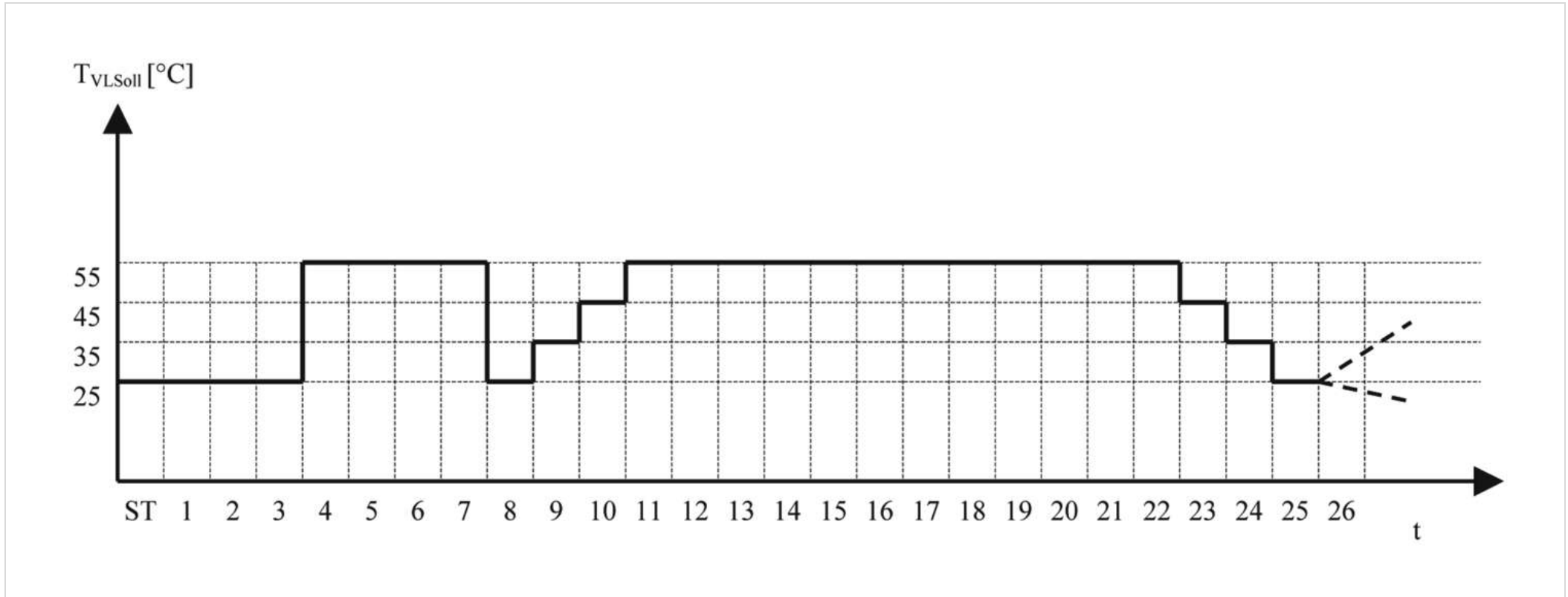
Fig. 52: Time sequence - functional heating with subsequent floor covering heating
