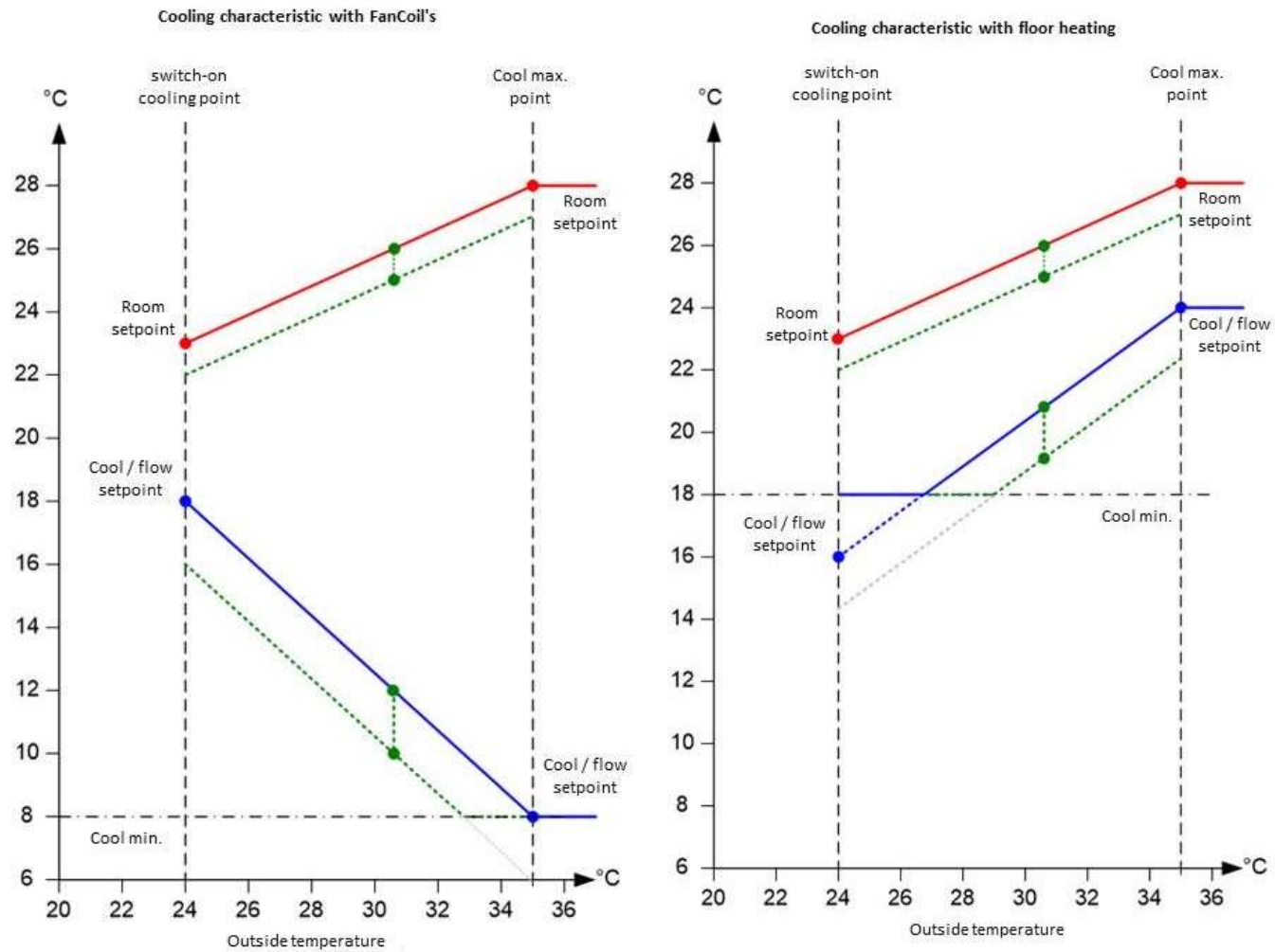
Fig. 44: Connection room Setpoint temperature ⇔ flow temperature
