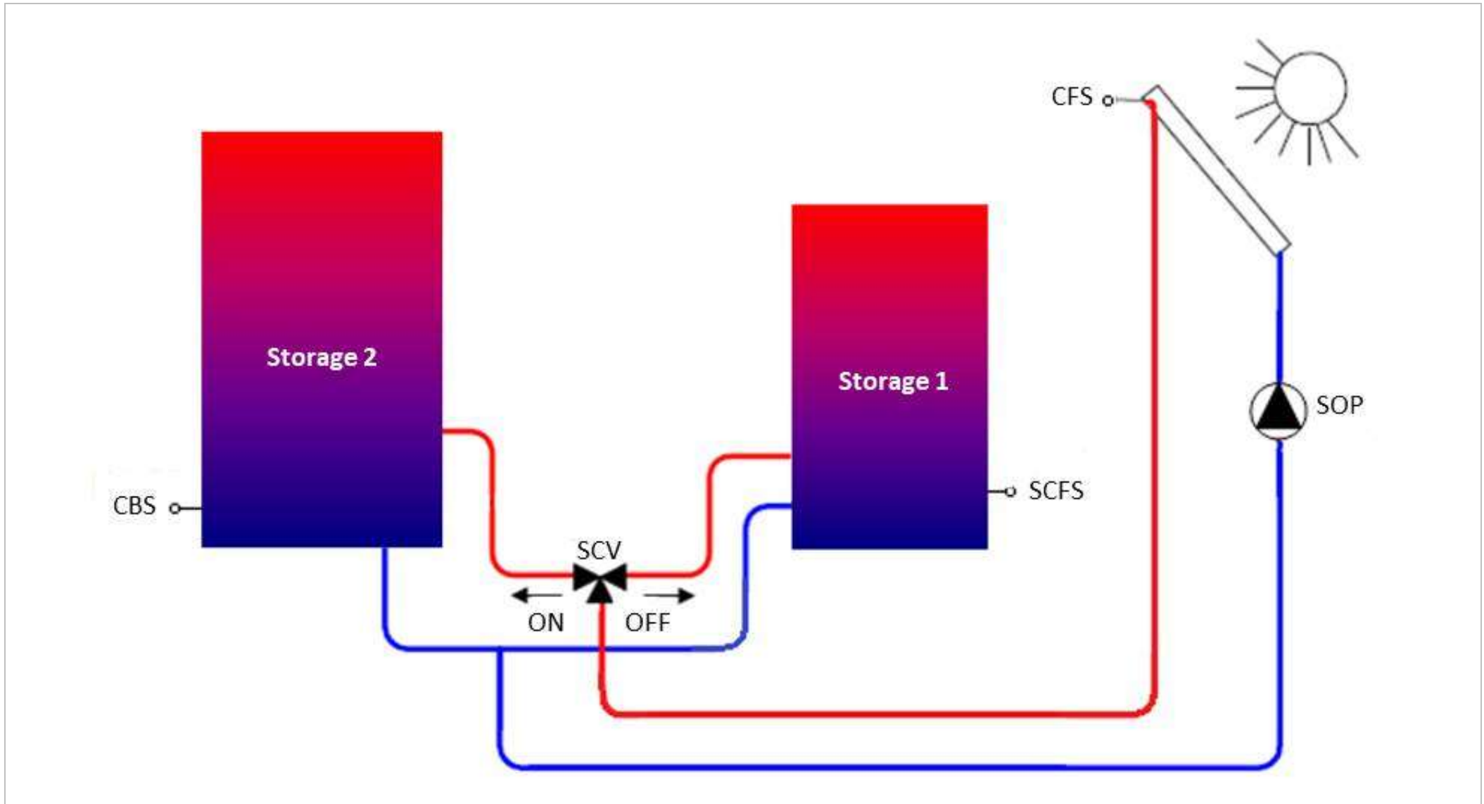
Fig. 63: Double buffer system of a solar thermal system (example)
