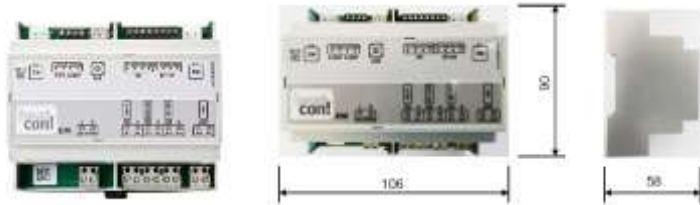
heatcon! Extension module EM 100 Article number 9600704000
