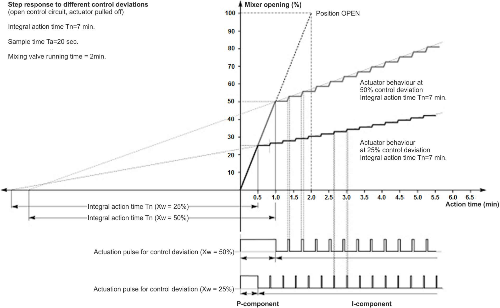
Fig. 41: Example for the interaction of the control parameters
