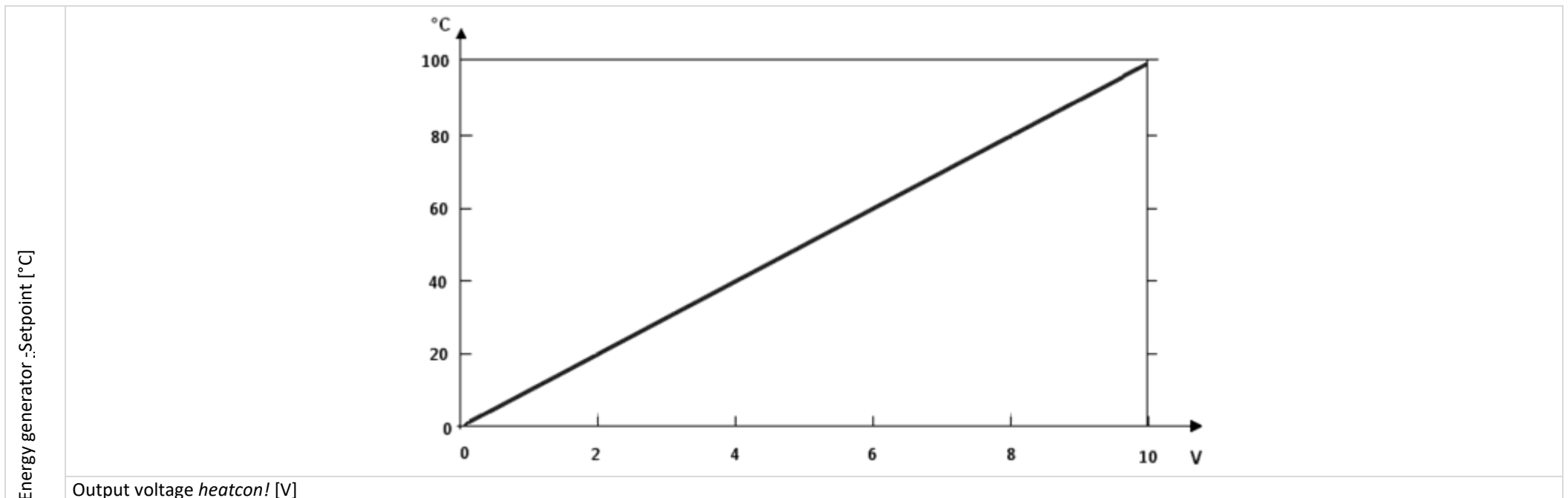
Fig. 35: Performance chart with adaptation to the energy generator
