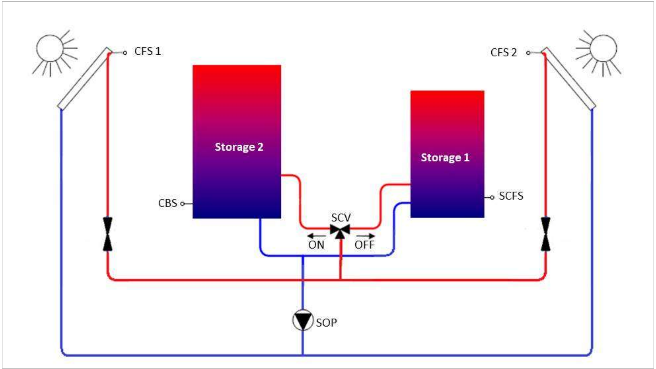
Fig. 65: Double collector system and double buffer system with charge valve switchover
