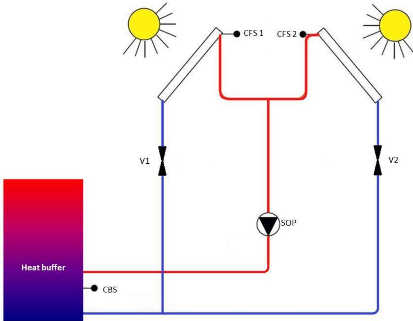
Fig. 64: Solar - double collector array (example)
