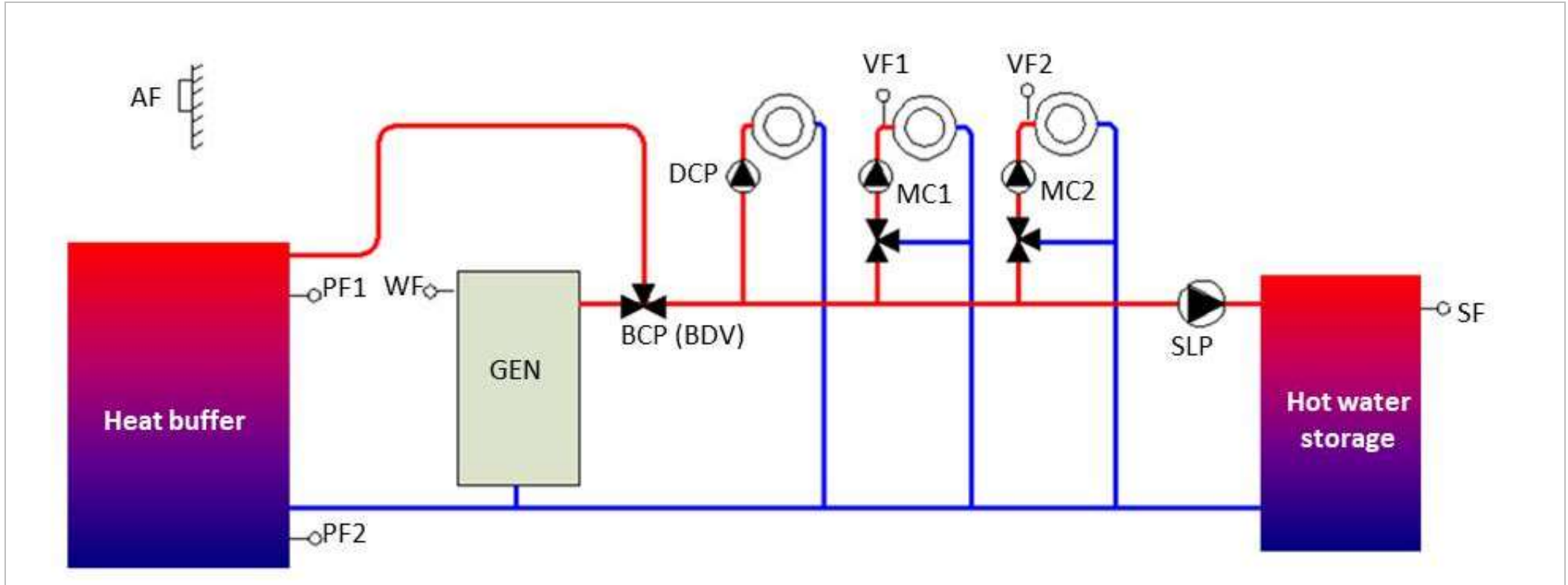
Fig. 60: Buffer discharge control to heating circuit and hot water
