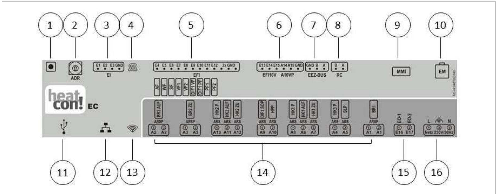
Fig. 30: heatcon! EC - connection assignment
