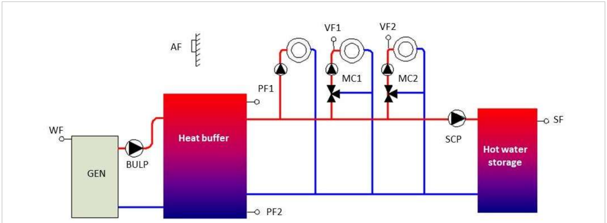
Fig. 55: Buffer charge control with heating circuit and hot water Requests
