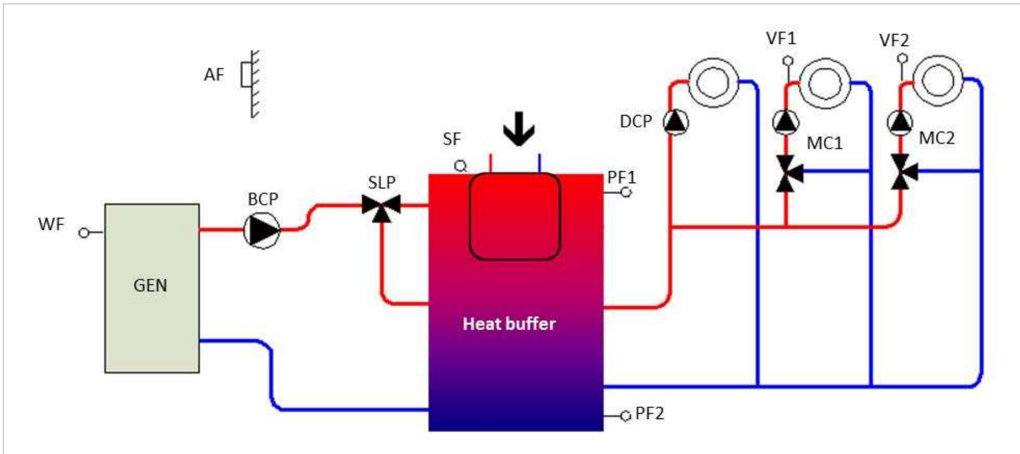
Fig. 59: Buffer charge control with hot water diverter valve
