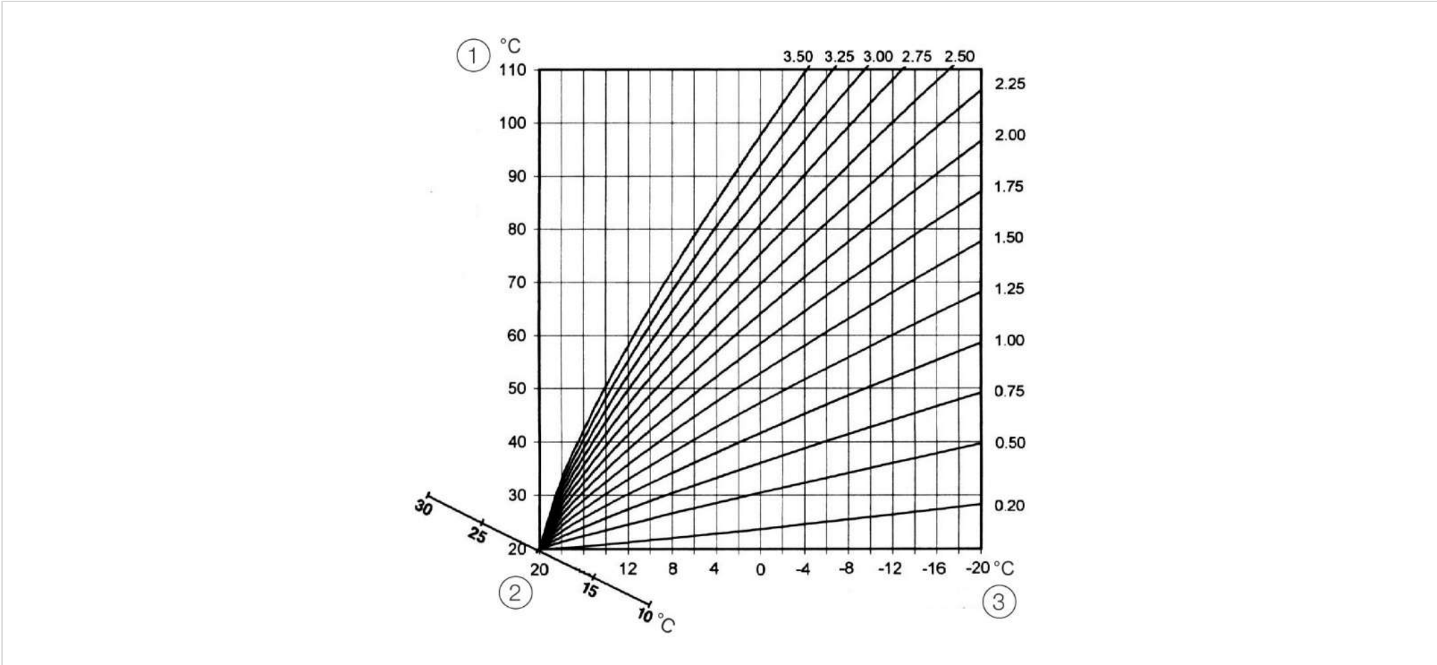
Fig. 44: Heating Characteristic Curve
