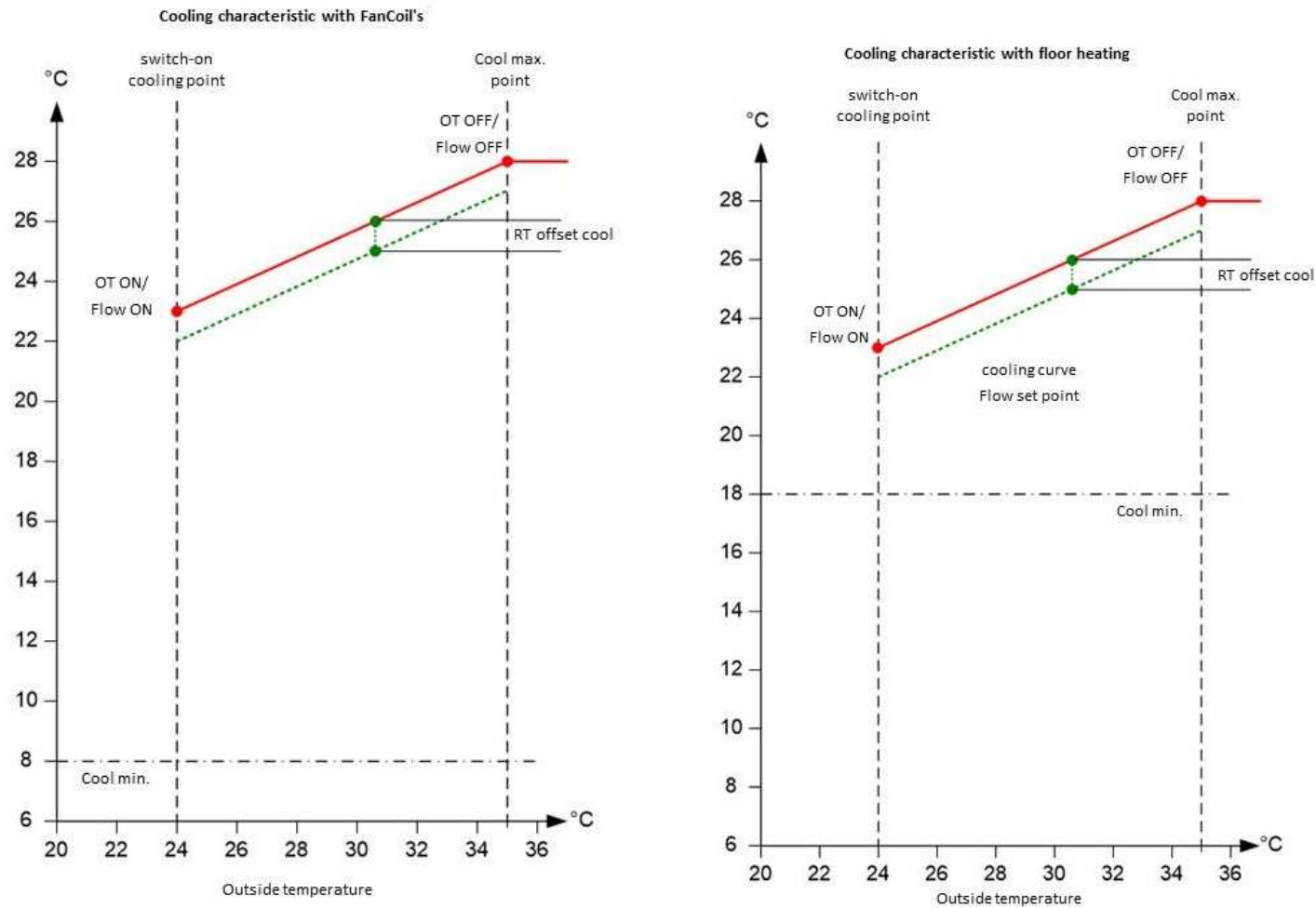
Fig. 40: Calculating room Setpoint temperature
