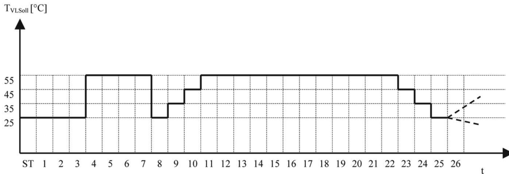
Fig. 49: Time sequence - functional heating with subsequent floor covering heating
