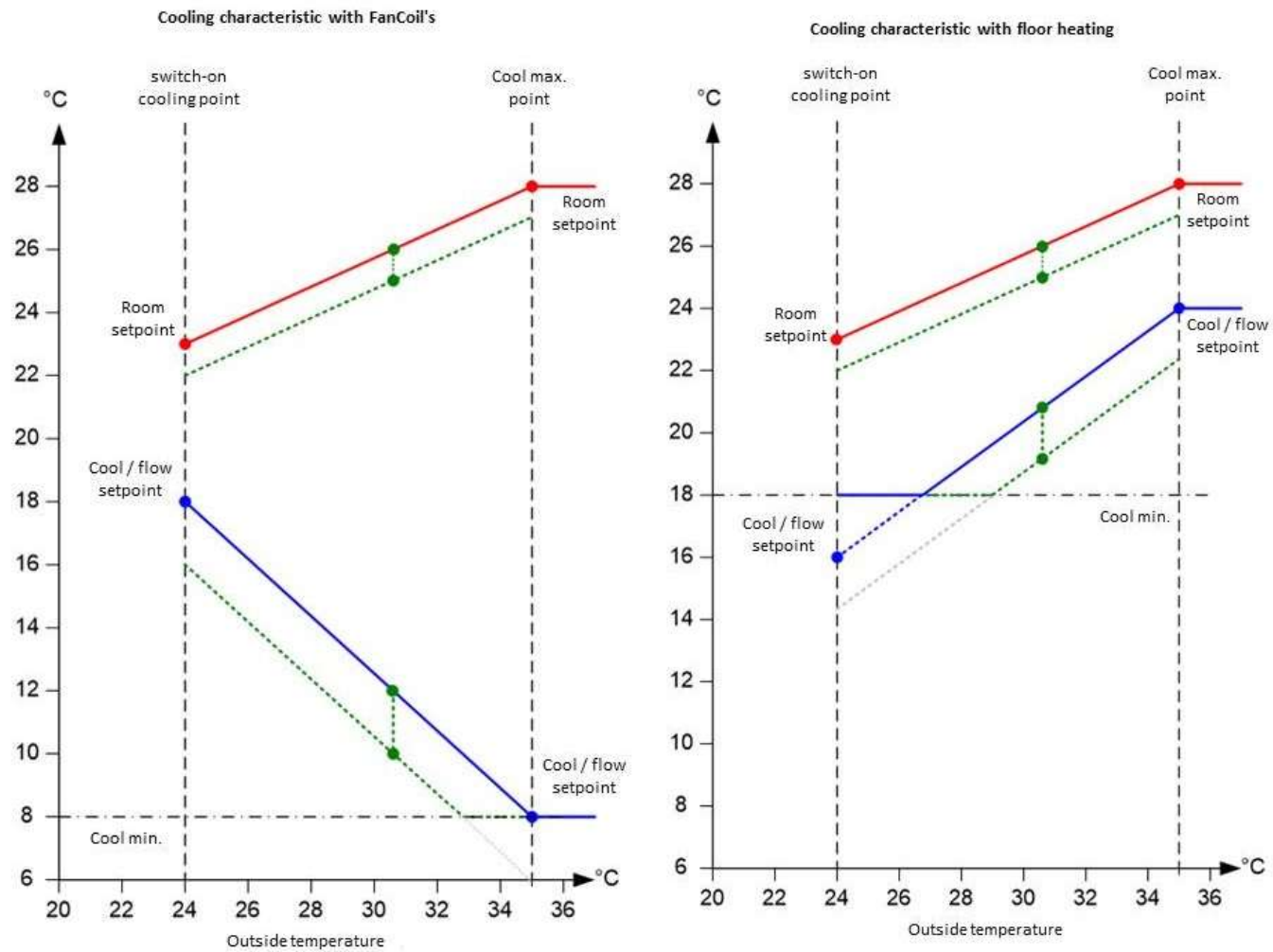
Fig. 41: Connection room Setpoint temperature ⇔ flow temperature
