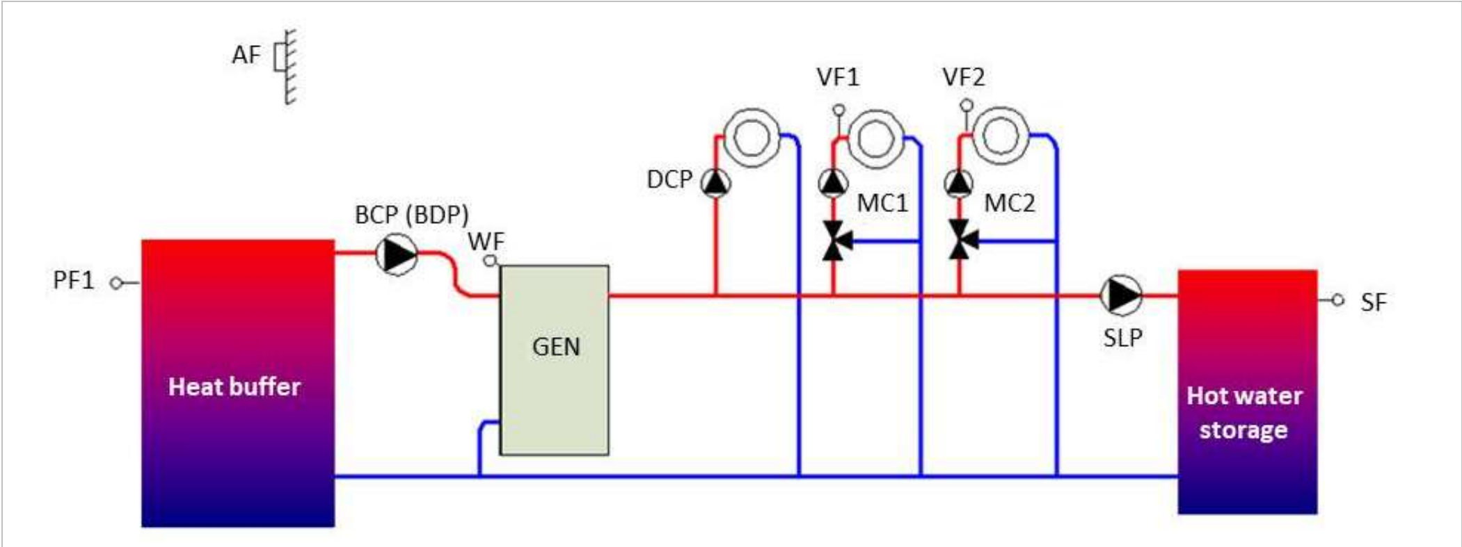
Fig. 59: Buffer discharge control type 2 on heat generator
