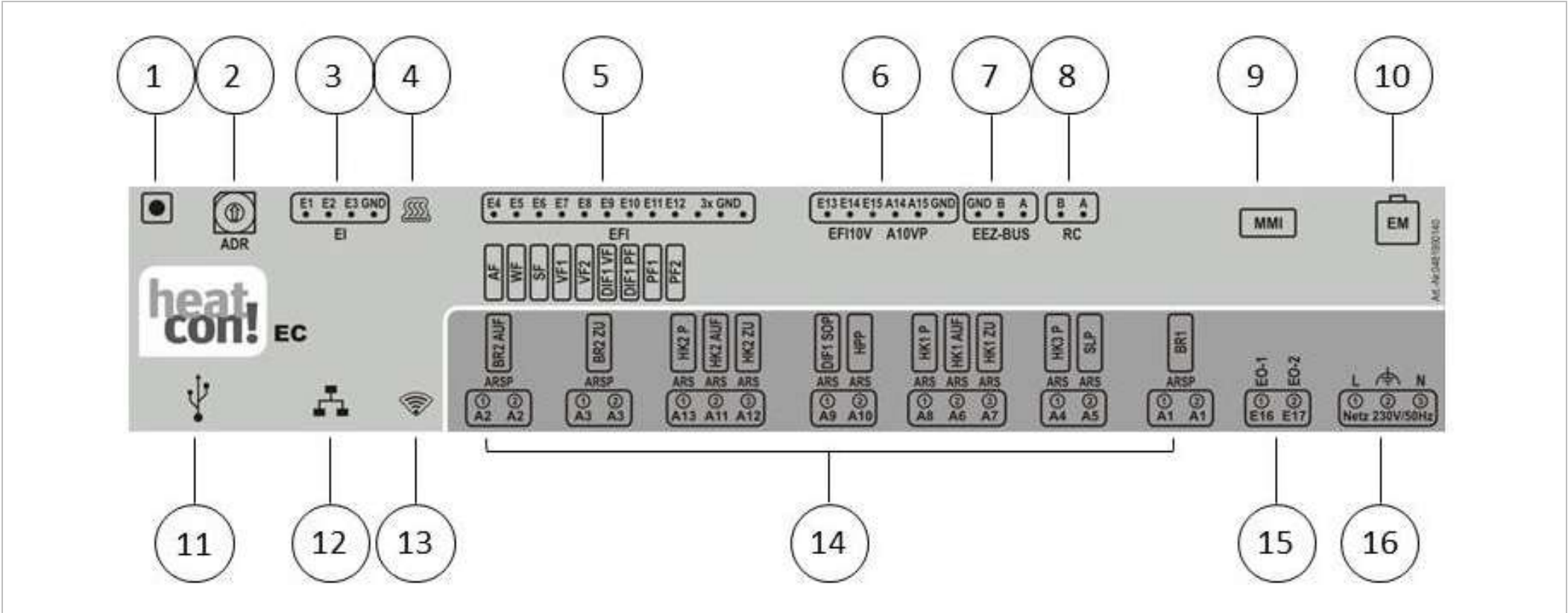
Fig. 27: heatcon! EC - connection assignment
