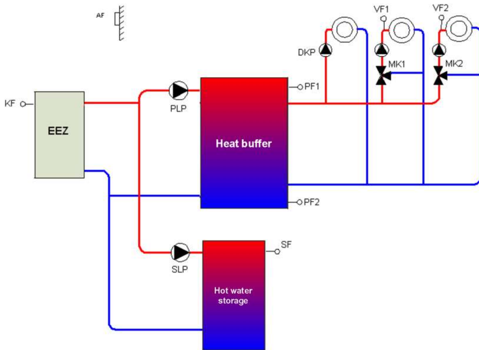
Fig. 55: Buffer charge control for heating circuit Request
