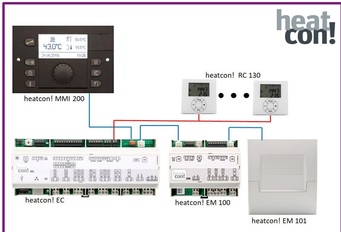
System overview
